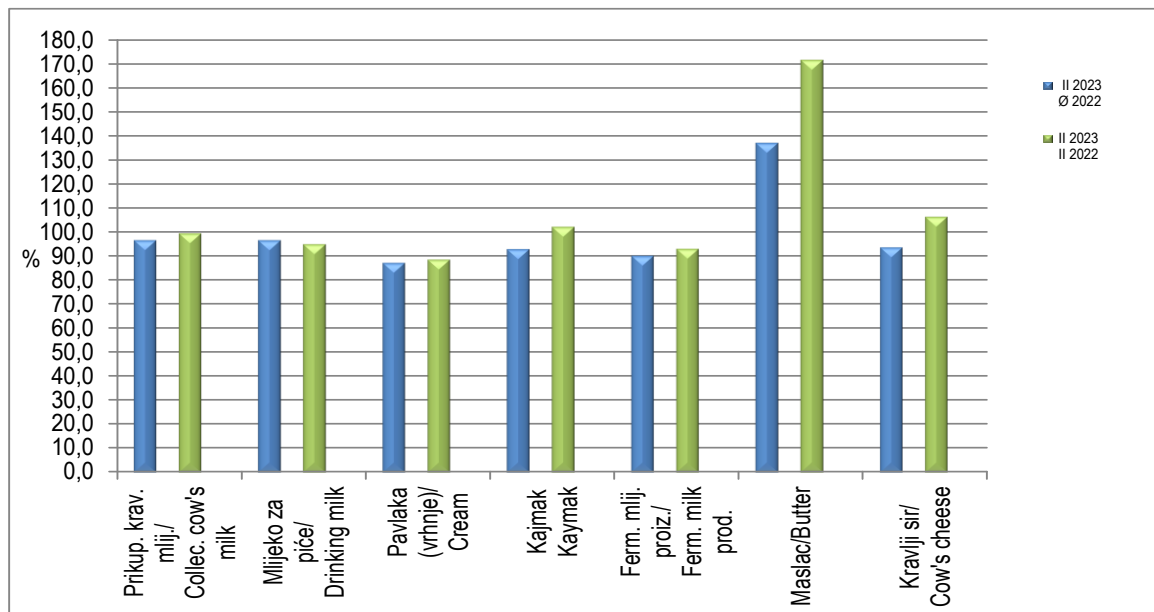
Graph 1. Indices of collected cow's milk and produced dairy products
