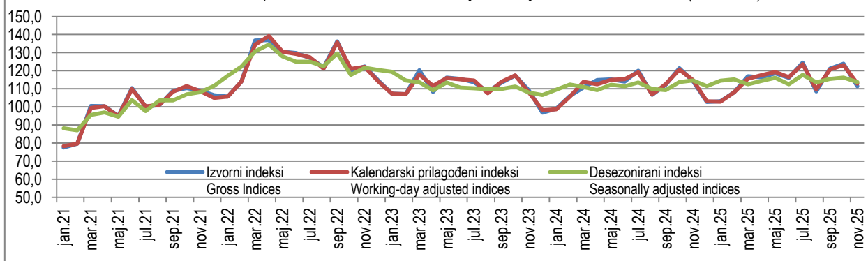
Grafik 1. Vremenska serija industrija ukupno: januar 2021 - novembar 2025. (2021.=100) Graph 1. Time series for Total industry: January 2021 - November 2025 (2021= 100)
