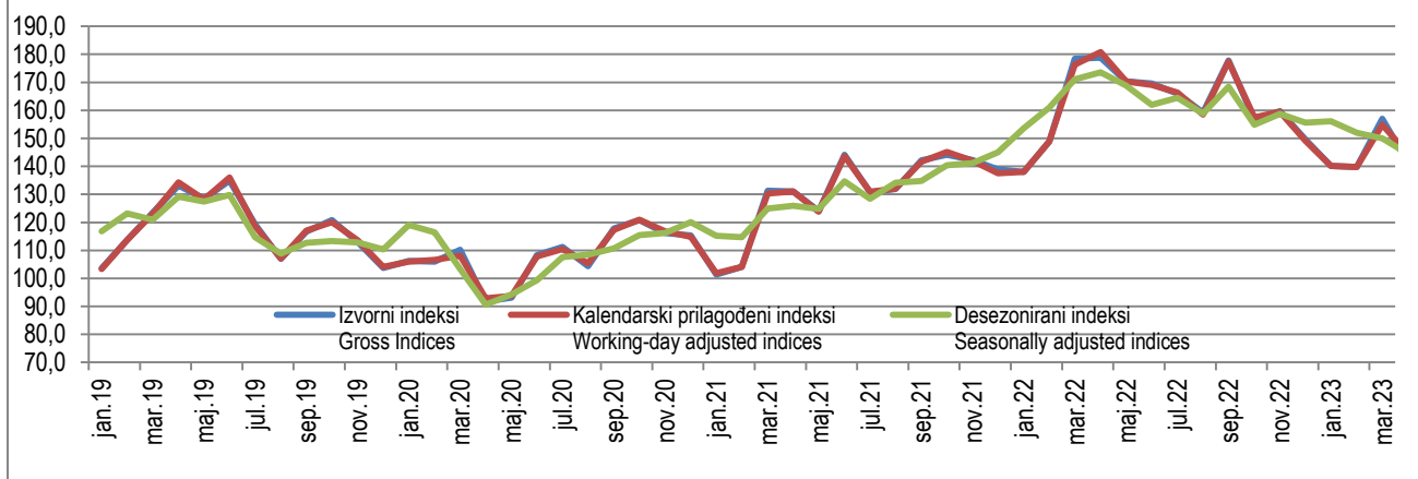
Grafik 1. Vremenska serija industrija ukupno: januar 2019 - april 2023. (2015.=100) Graph 1. Time series for Total industry: January 2019 - April 2023 (2015 = 100)
