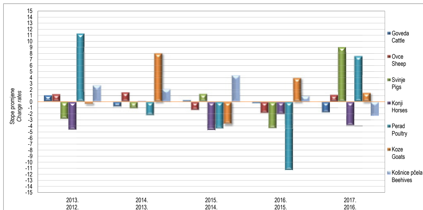
Graph 1. Yearly change rates calculated from indices of number of livestock and poultry
